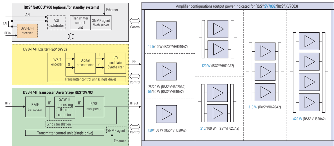
System block diagram of the Transmitter/Retransmitter R&S®SV7002 and Transposer/Gap Filler R&S®XV7003
